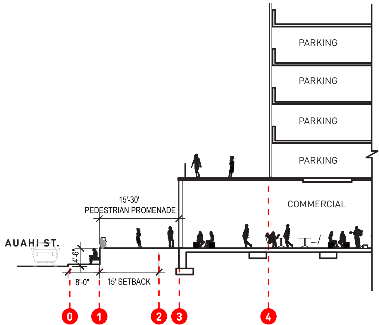
1. Ko'ula terraced podium - cross section
